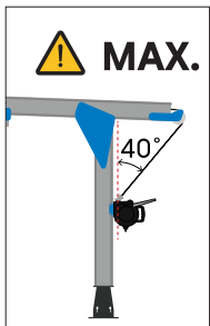
Maximum angle allowance is 40° from vertical
