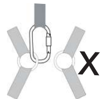
fig 6 - Incorrect fastening of chest loops
