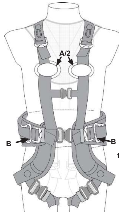
fig 4 - front attachment points
